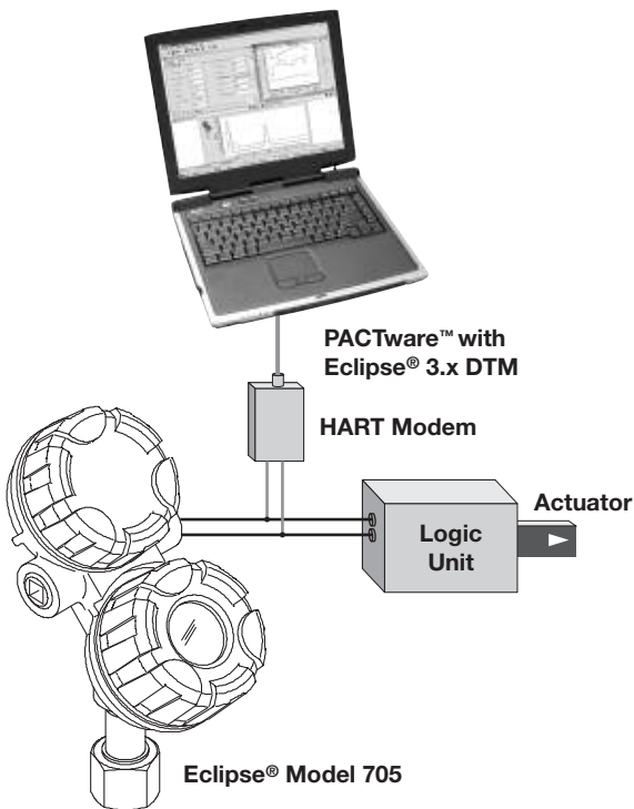
Figure 1 Typical System
