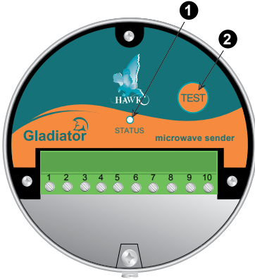
G1S Sender
