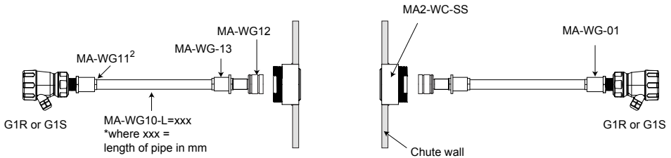
2 Displayed drawing includes qty 3 of MA-WG11 locking nut per side
