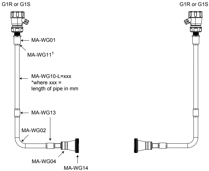
1 Displayed drawing includes qty 5 of MA-WG11 locking nut per side
