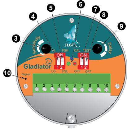
G1R Receiver
