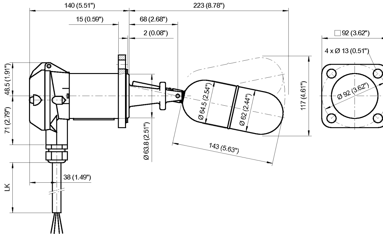
U3...: Submersible level switch with 3 m cable
